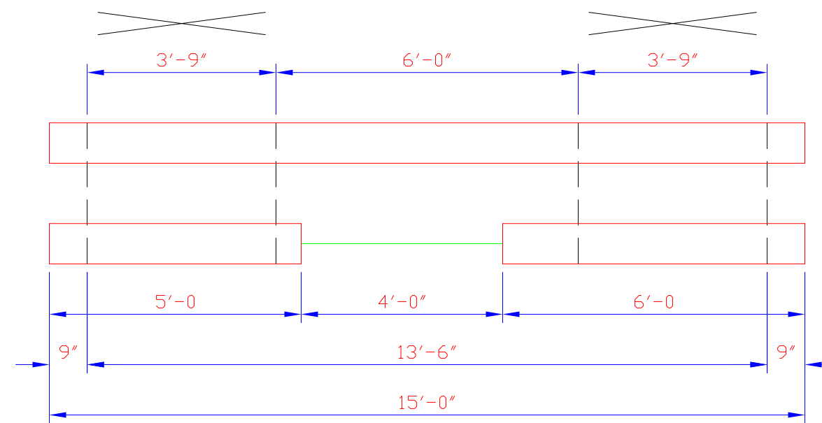
PLAN OF BLEACHER (1/4 SCALE)
