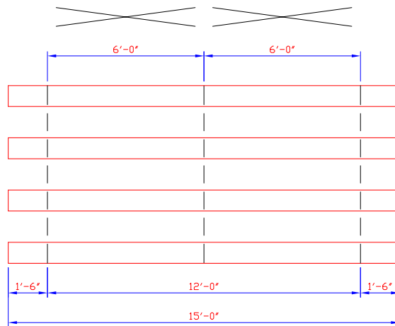
PLAN OF BLEACHER (1/4 SCALE)
