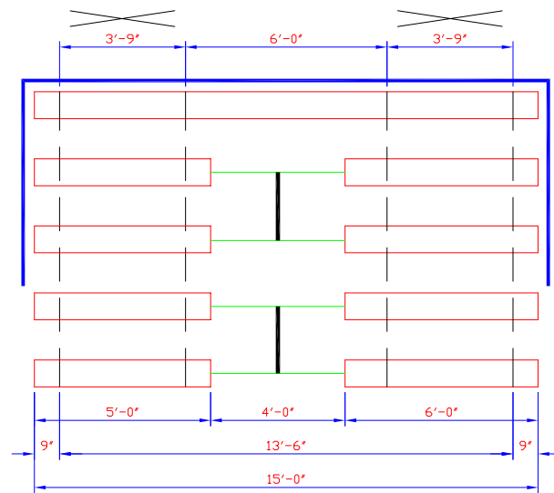
PLAN OF BLEACHER
