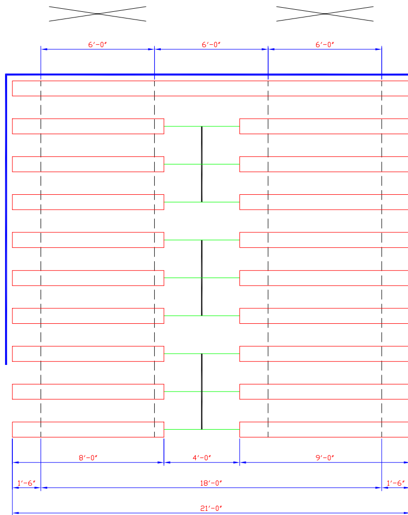
PLAN OF BLEACHER
