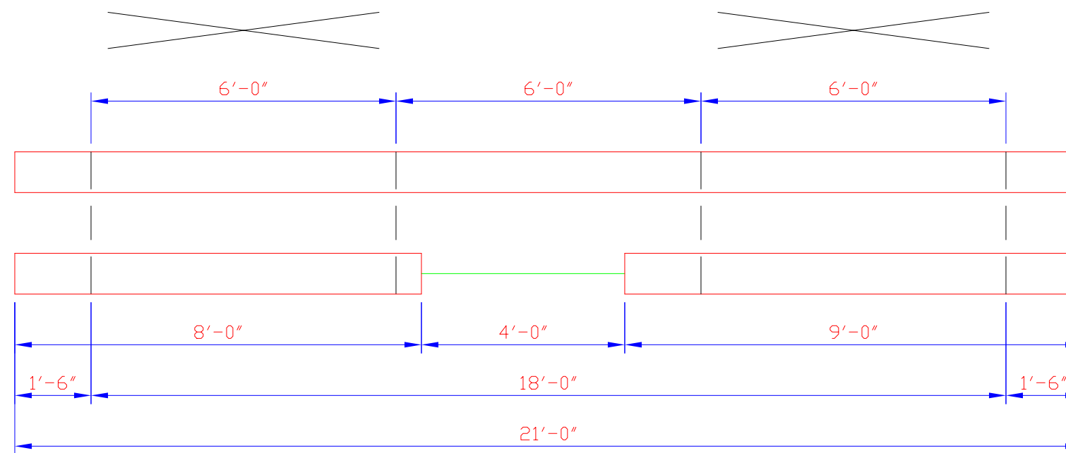
PLAN OF BLEACHER (1/4 SCALE)
