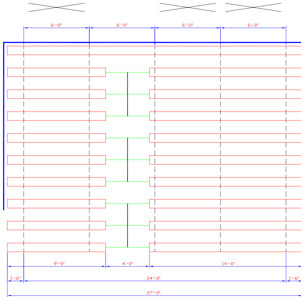
PLAN OF BLEACHER
