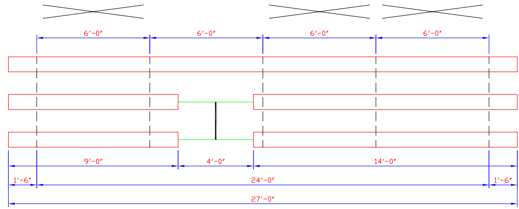
PLAN OF BLEACHER (1/4 SCALE)
