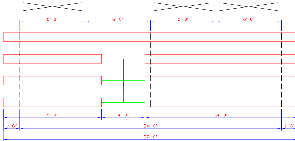
PLAN OF BLEACHER (1/4 SCALE)
