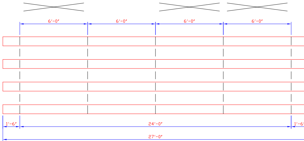
PLAN OF BLEACHER (1/4 SCALE)
