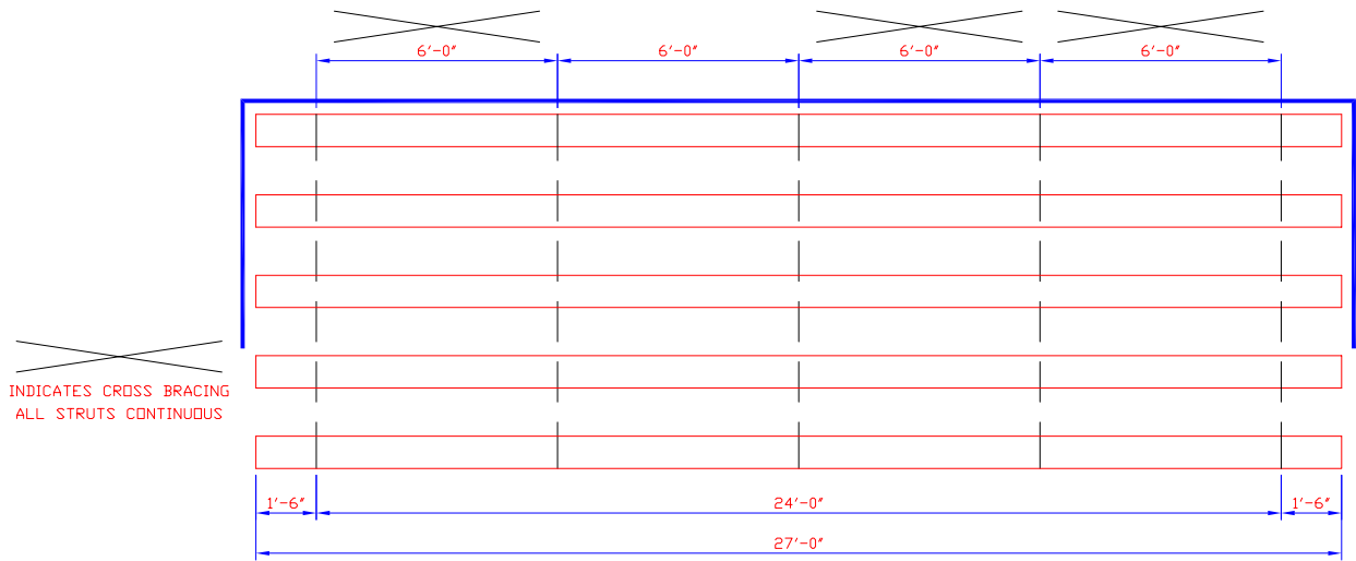
PLAN OF BLEACHER 1/2 SCALE
