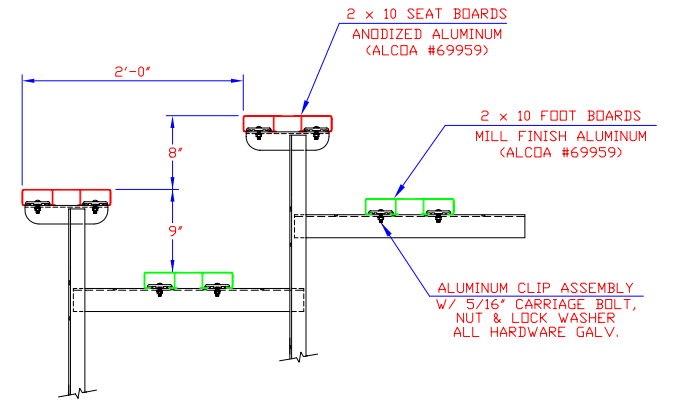
PLANK ARRANGEMENT FULL PLANK DECK SERIES
