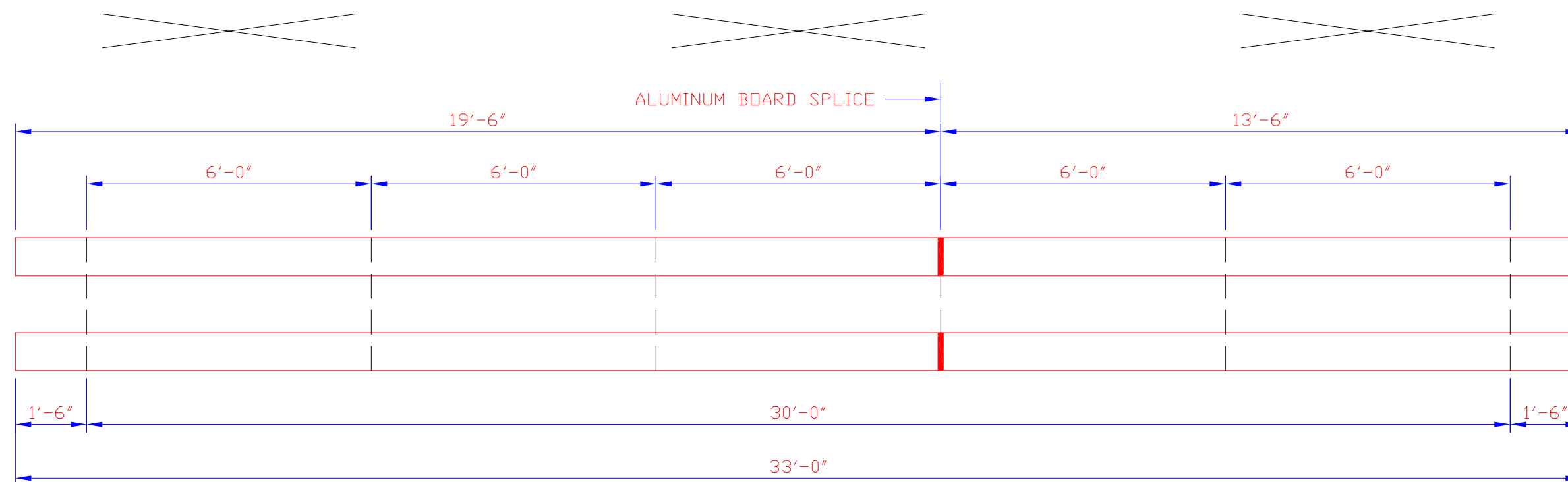
PLAN OF BLEACHER (1/4 SCALE)
