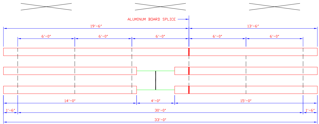
PLAN OF BLEACHER (1/4 SCALE)
