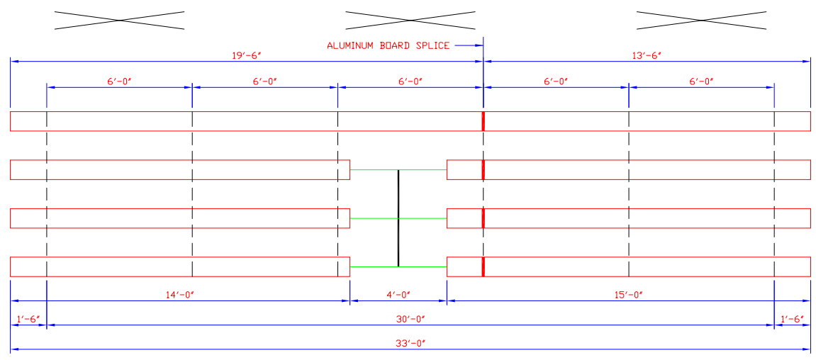
PLAN OF BLEACHER (1/4 SCALE)
