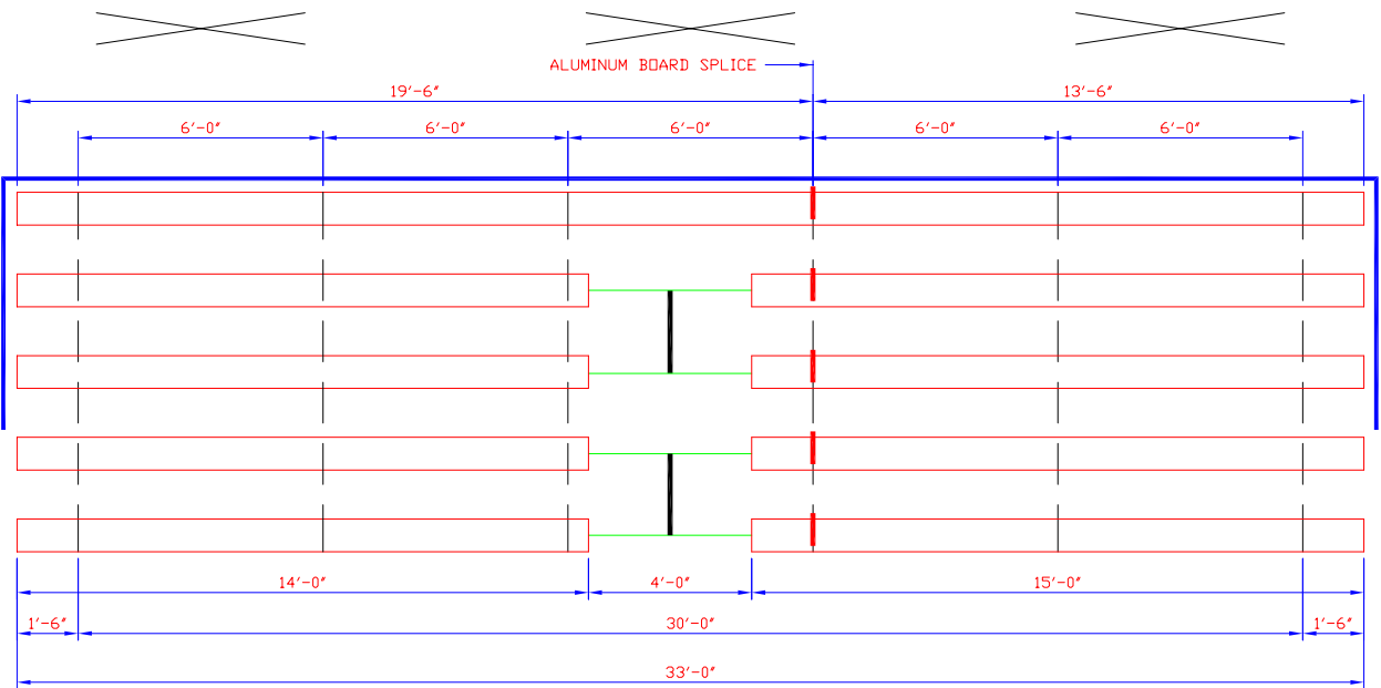
PLAN OF BLEACHER 1/2 SCALE
